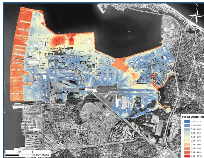
100 year storm with 2.0m sea level rise. Source: Kelly A. Burkes-Copes
